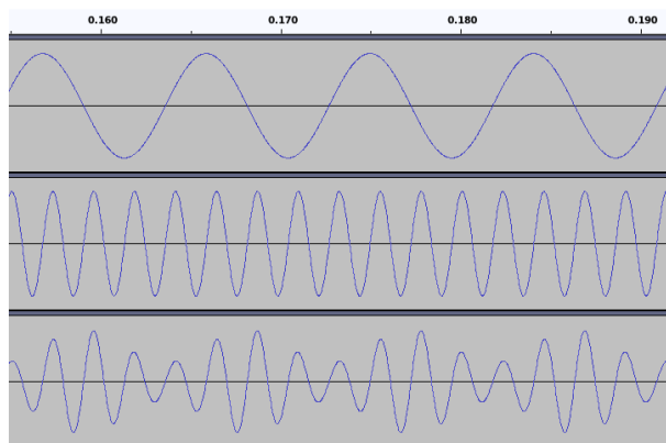
Figure 276: Example of AM Synthesis
